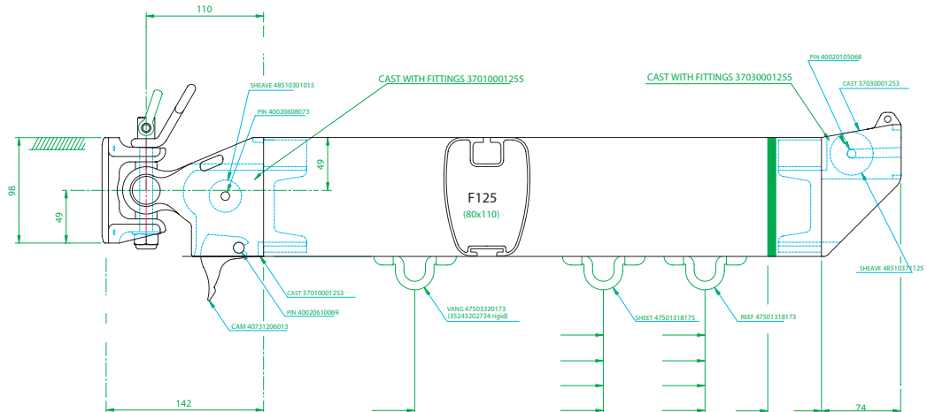
COMPLETE GOOSENECK 3451177OC15
