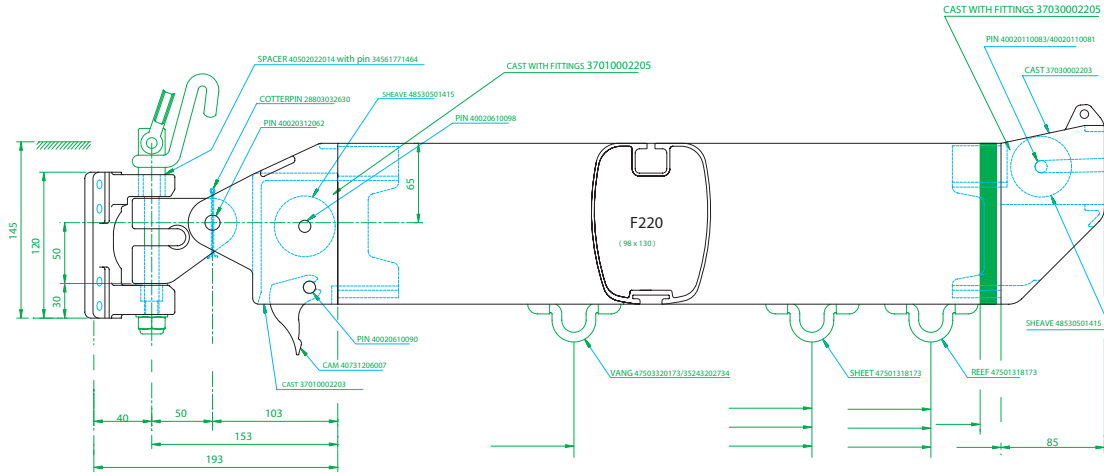
COMPLETE GOOSENECK 34511770C25
