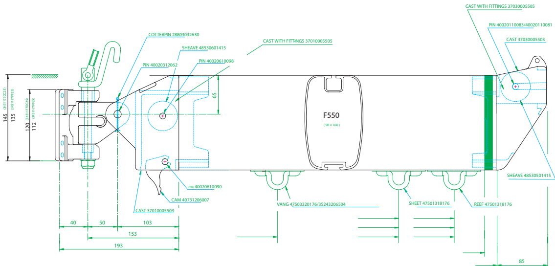
COMPLETE GOOSENECK 34511770C26 / or / 34511779F25
