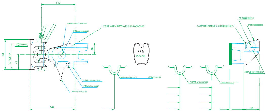
COMPLETE GOOSENECK 3451177OC05
