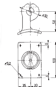
36031300498 Rotating mast step for profiles F32C and F49C.
